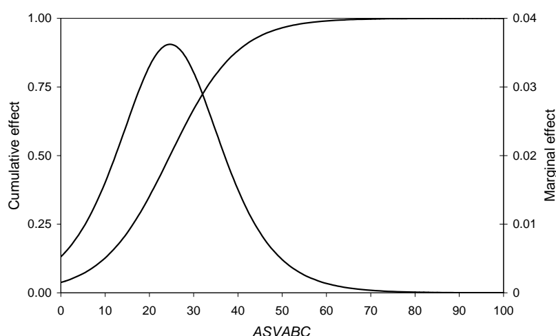
Figure 10.5 Cumulative and marginal effects of ASVABC
