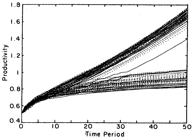
FIGURE 6C. Graph of 100 runs ( \mu = 0.15 )
