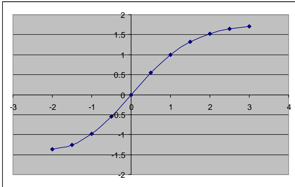
Figure 3 Characteristic-Beta Function for the Size Characteristic
