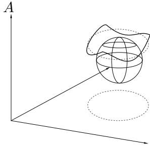
Fig. 2: Spatial agglomeration on 3-dimensional globe Figure shows a horizontal slice through the local perturbations that converge back to steady state only with clusters in the spatial distribution
