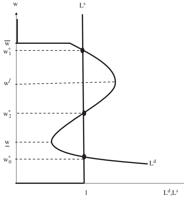
Fig. 2. Multiple equilibria.
